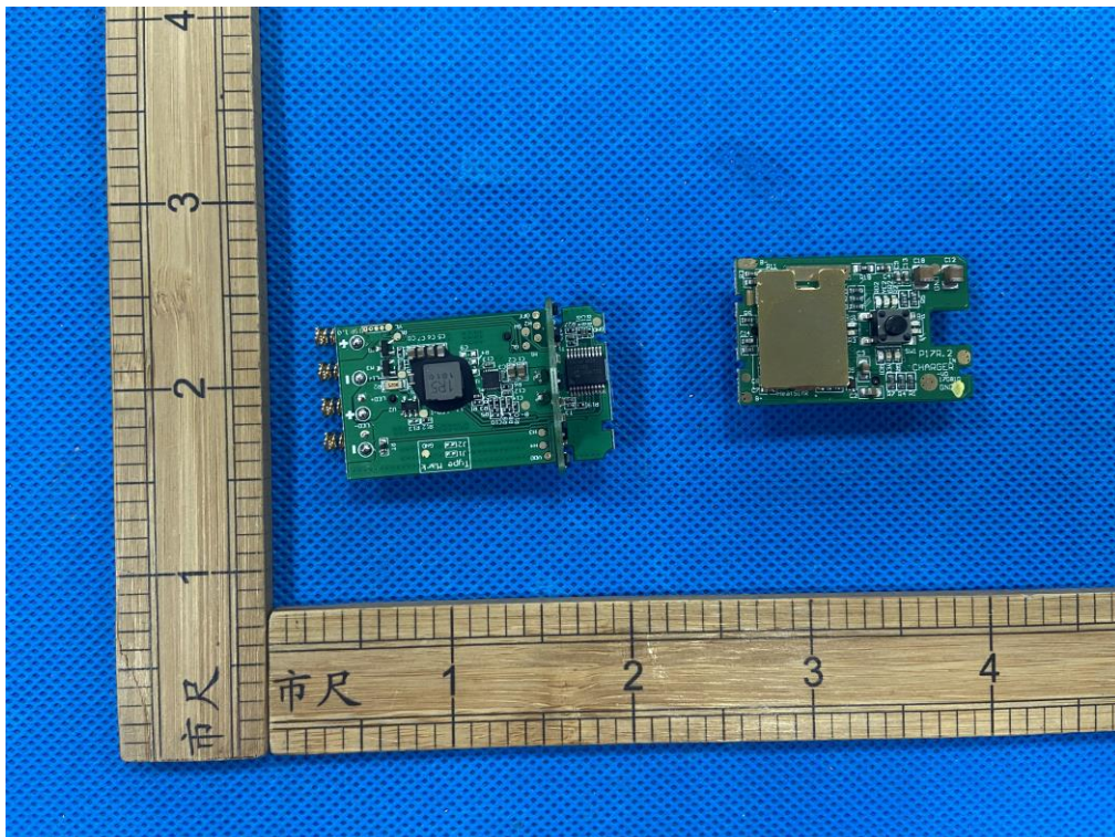
Figure 12. Bottom view of Control board PCB
