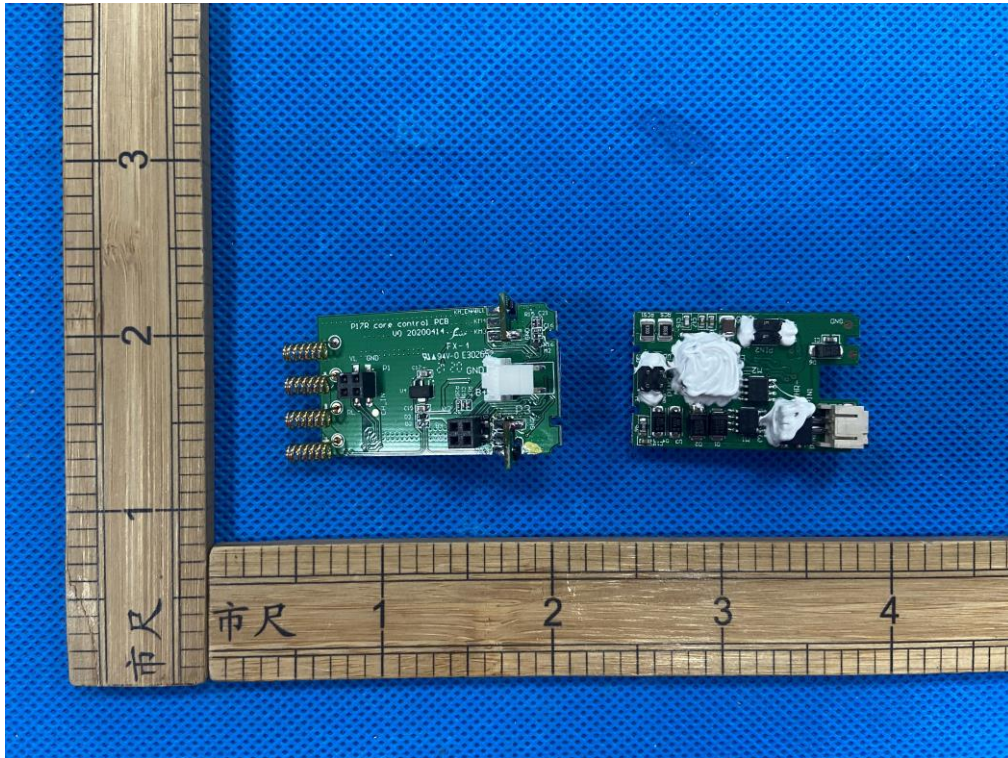
Figure 11. Top view of Control board PCB
